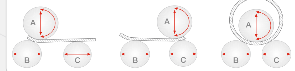
3 rolls bending machine with variable pitch model EMO
